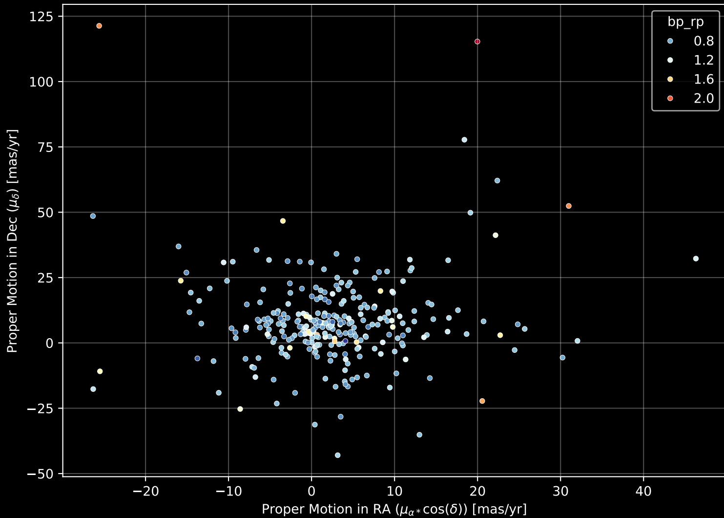
GALAH DR4 Field: [989] Proper Motion Diagram (n= 290)
