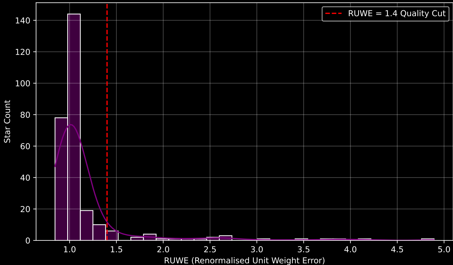
GALAH DR4 Field [989] RUWE Distribution (n= 278)
