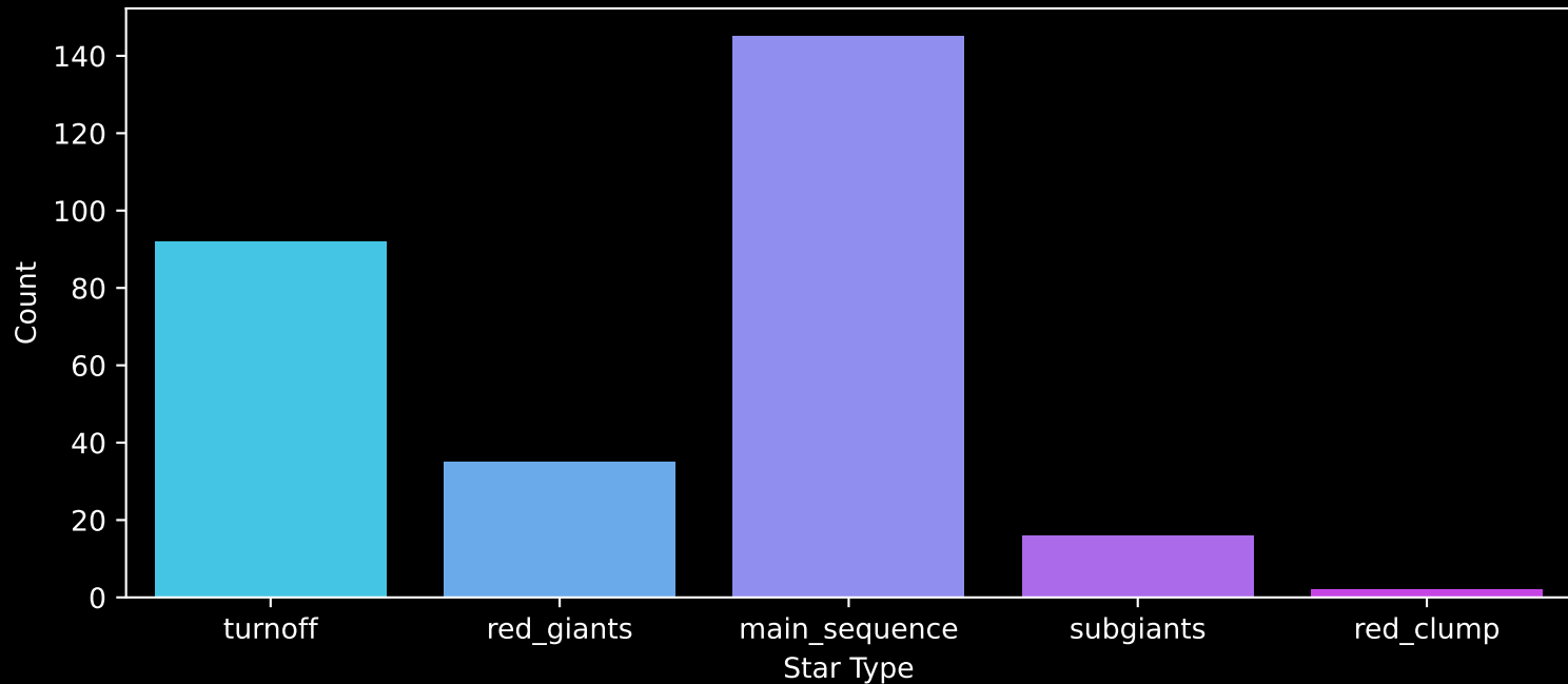
GALAH DR4 Field: [989] Count plot of Star Type
